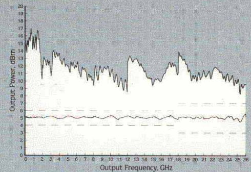
Figure 2: A composite plot of maximum available power and leveled output power from a typical Giga-tronics Model 1026. Dotted lines indicate specified accuracy and flatness tolerance of leveled output.
